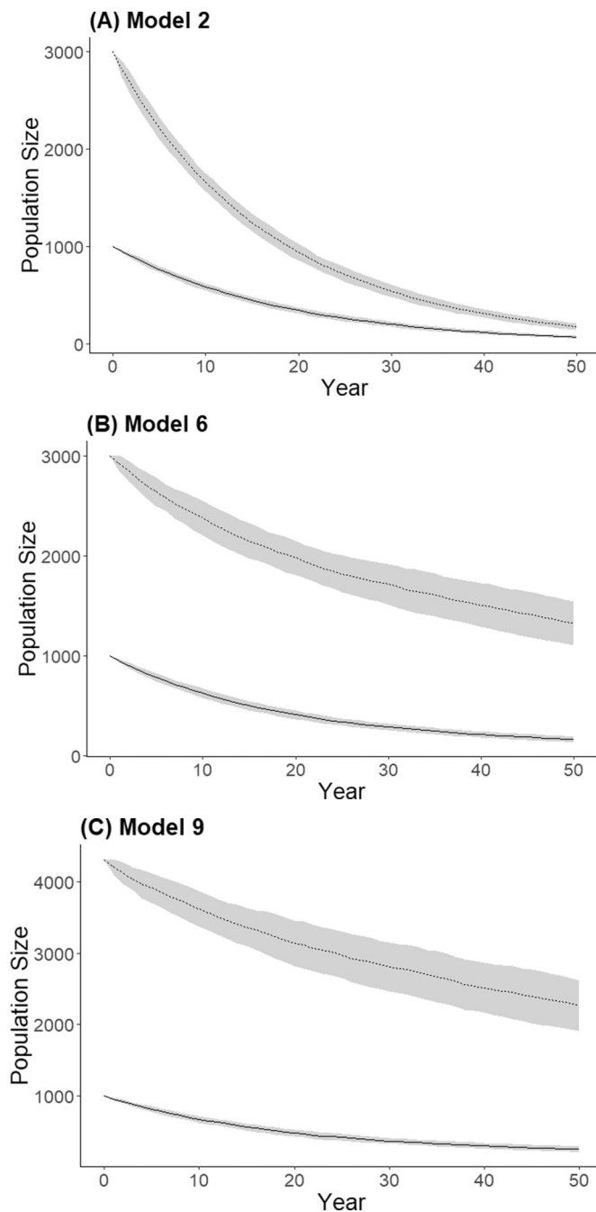
Fig. 3. A selection of predicted population trajectories for Iron/McIllwraith population and the meta-population. The reference year (Year 0) is 2018. In all models, upper (dotted) line = meta-population and lower (unbroken) line = Iron/McIllwraith population. Standard deviations, shown as ribbons, are given for each year of predictions. Model 2 shows dispersal adjusted for landscape permeability. Model 6 is based on Model 2 but allows higher reproductive success outside the Iron/McIllwraith Ranges. Model 9 is based on Model 6 but has a larger Central/west population. See Table 5 for full descriptions of the models.
